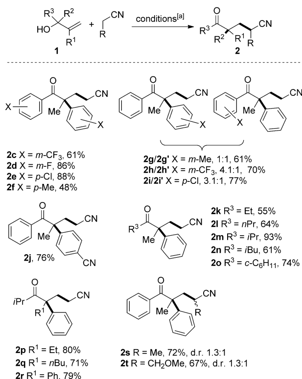
Scheme 2. Scope of the copper-catalyzed coupling reaction of allylic alcohols with alkyl nitriles. [a] Reactions were carried out on a 0.05 mmol scale in a sealed tube. Reaction conditions: Cu(OTf) 2 (0.5 equiv), 1,10-Phen (0.5 equiv), DTBP (4.0 equiv, added in two portions), Na 3 PO 4 (2.0 equiv), RCH 2 CN (solvent, 0.1 M), N 2 atmosphere, 140 °C.
